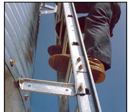
Sidewall Ladders have round rungs with a raised, non-skid surface and are permanently attached to the ladder rail for a hand-filling, secure grip.
