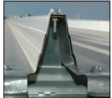
High-Rise Roof Rib is a full 3 inches (76 mm) tall, utilizing Brock's strength-giving 3-step rib design.
